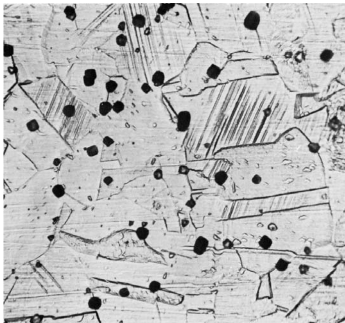
FIG. 7 End Grain Pitting II (500 \times )
