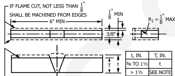
FIG. A2.13 Transverse Face- and Root-bend Test Specimens
