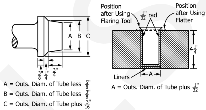
FIG. A2.10 Crush Test Specimen
