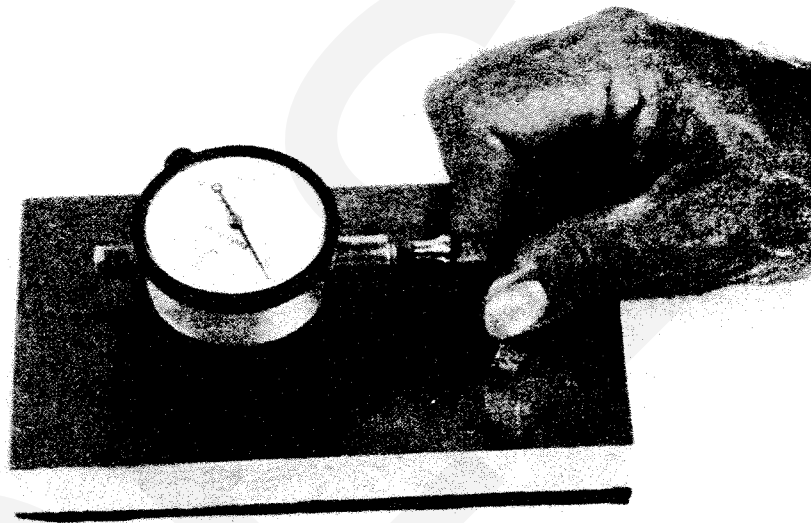
FIG. 16 LATERAL EXPANSION GAGE FOR CHARPY IMPACT SPECIMENS
