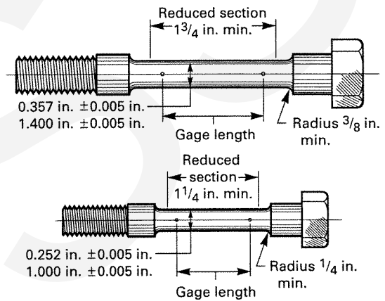
FIG. A3.3 TENSION TEST SPECIMEN FOR BOLT WITH TURNED-DOWN SHANK
