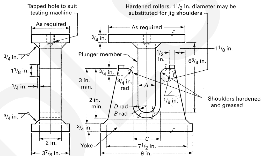
FIG. A2.14 SIDE-BEND SPECIMEN FOR FERROUS MATERIALS
