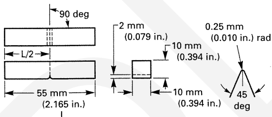
(a) Standard Full Size Specimen
