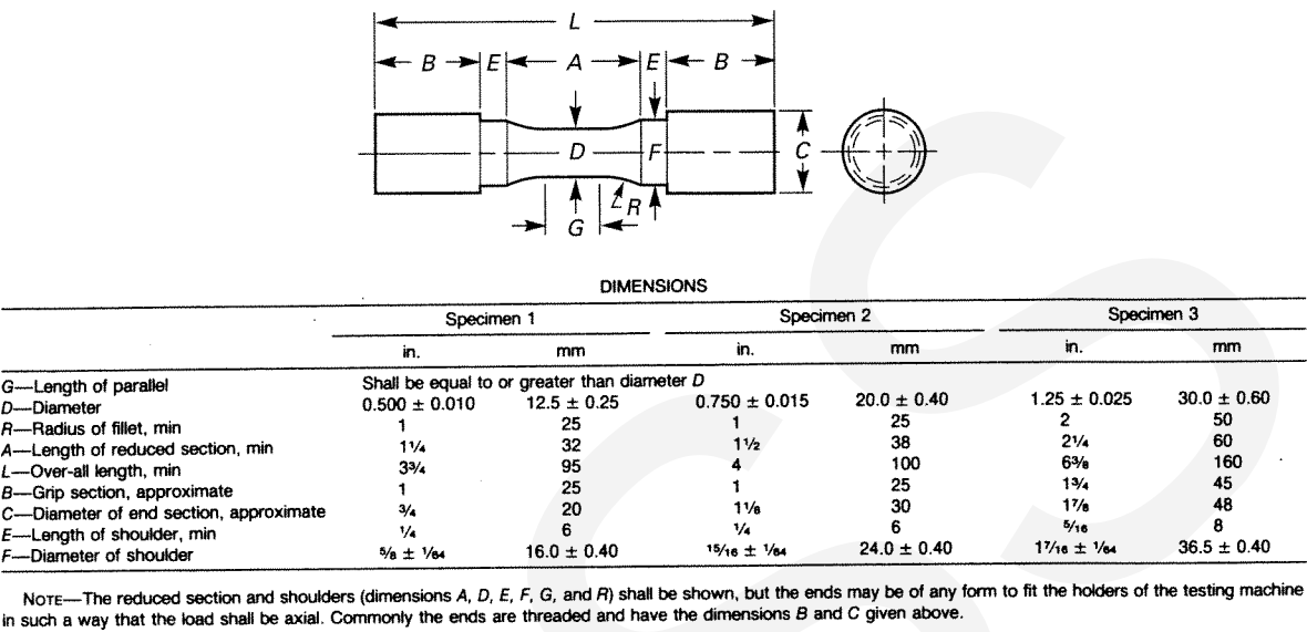
FIG. 6 STANDARD TENSION TEST SPECIMENS FOR CAST IRON
