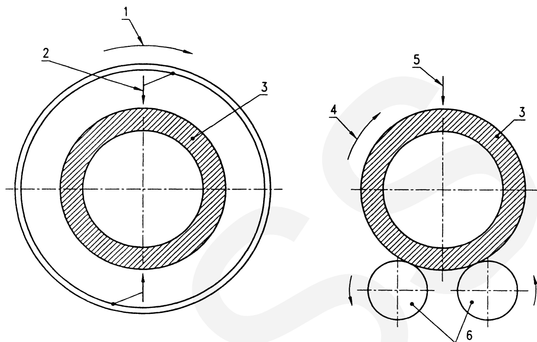
a) Rotating pancake coil technique (linear movement through rotating pancake coil assembly)
