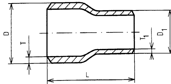
Figure 5 — Concentric reducer - Form 2
