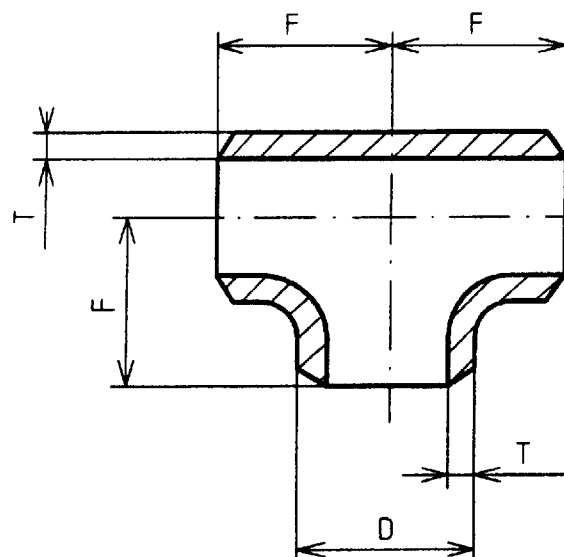
Figure 7 — Equal tee
