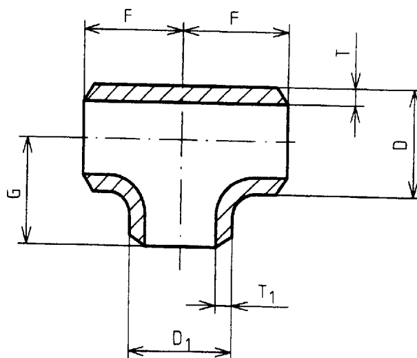
Figure 8 — Reducing tee
