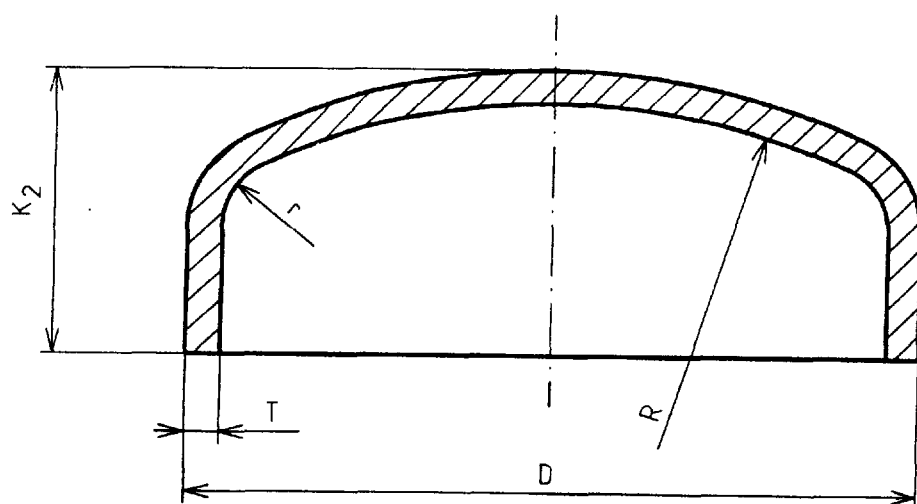
Figure 10 — Cap
