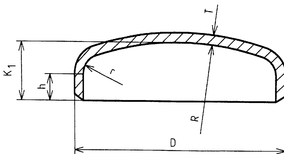
Figure 9 — Dished end
