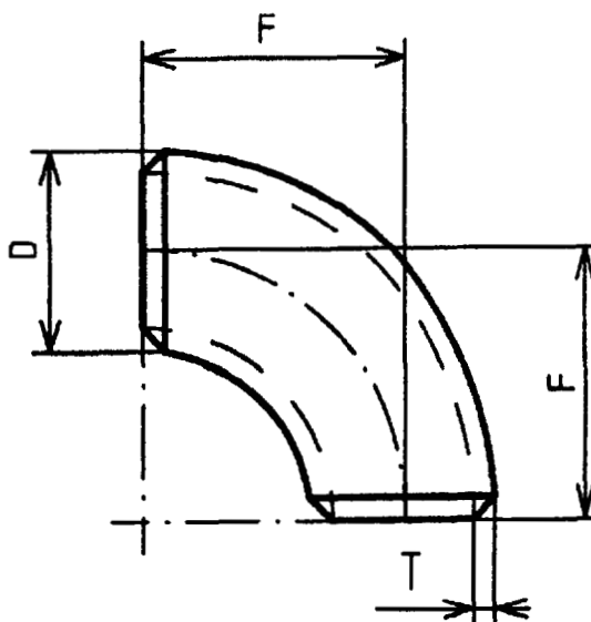
Figure 2 — 90° Elbow
