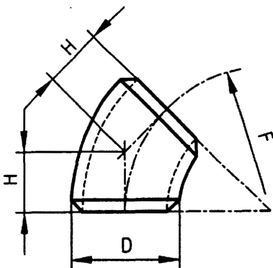
Figure 1 — 45° Elbow
