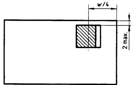
b) Where w > 50 \text{ mm} and t \leq 50 \text{ mm}
