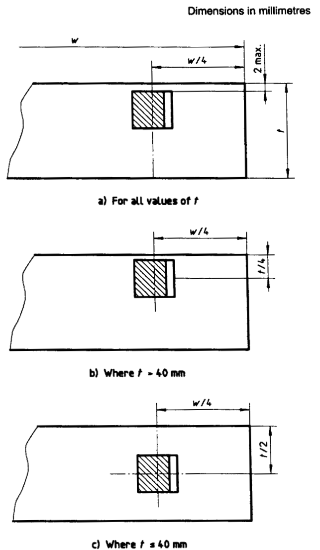
Figure A.11 — Flat products — Location of test pieces for impact testing (see A.6.2)
