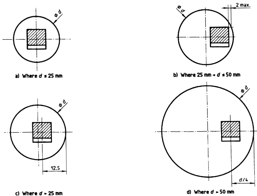
Figure A.5 -- Round bar and rod — Location of test pieces for impact testing (see A.3.2)
