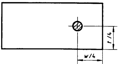
f) Round test piece where w \leq 50 mm and t > 50 mm
