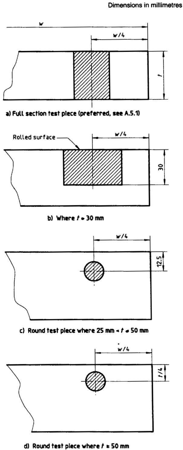
Figure A.10 — Flat products — Location of test pieces for tensile testing (see A.6.1)
