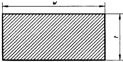
a) Full section test piece (wherever possible) see A.5.1
