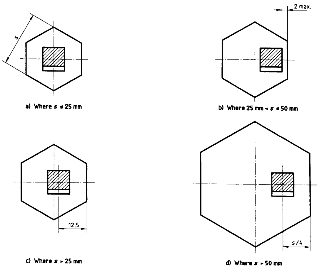
Figure A.7 — Hexagonal bar — Location of test pieces for impact testing (see A.4.2)
