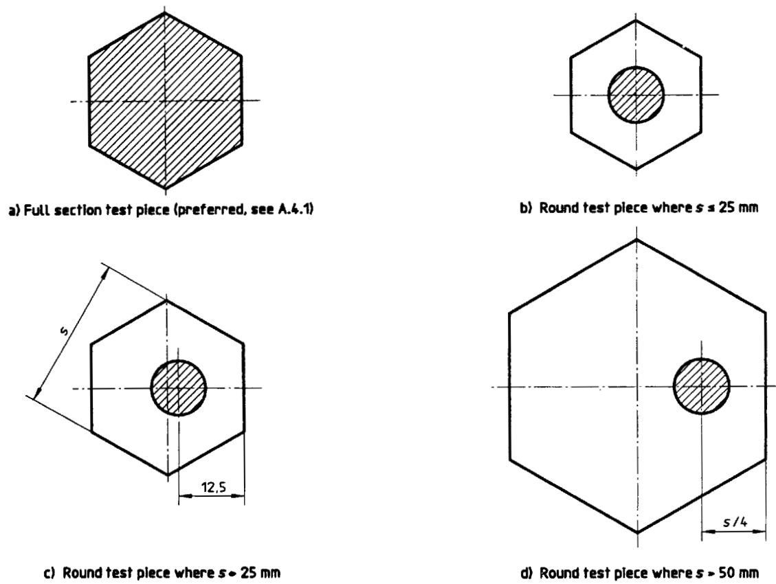
Figure A.6 — Hexagonal bar — Location of test pieces for tensile testing (see A.4.1)
