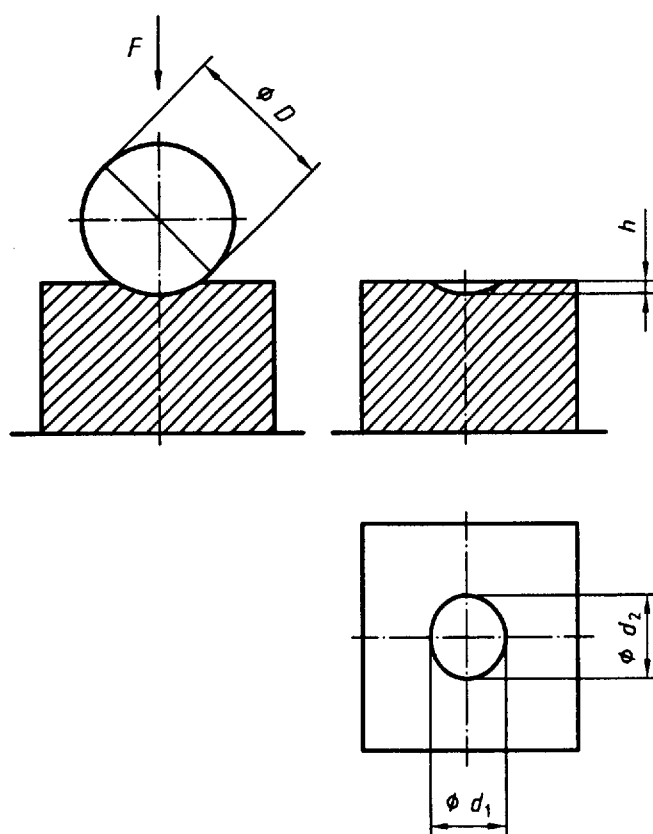
Figure 1 — Principle of test
