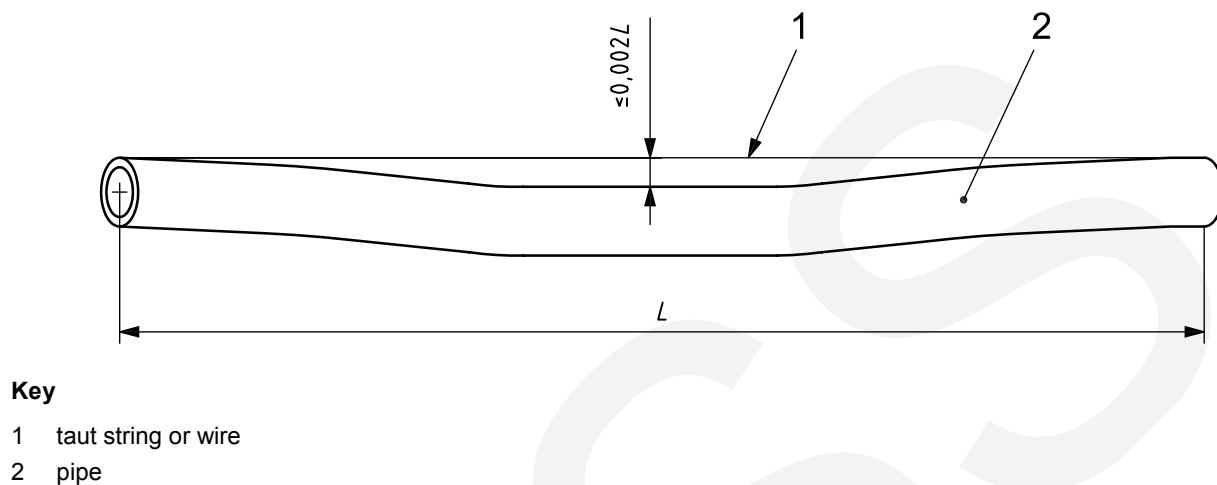
Figure B.1 — Measuring full-length straightness
